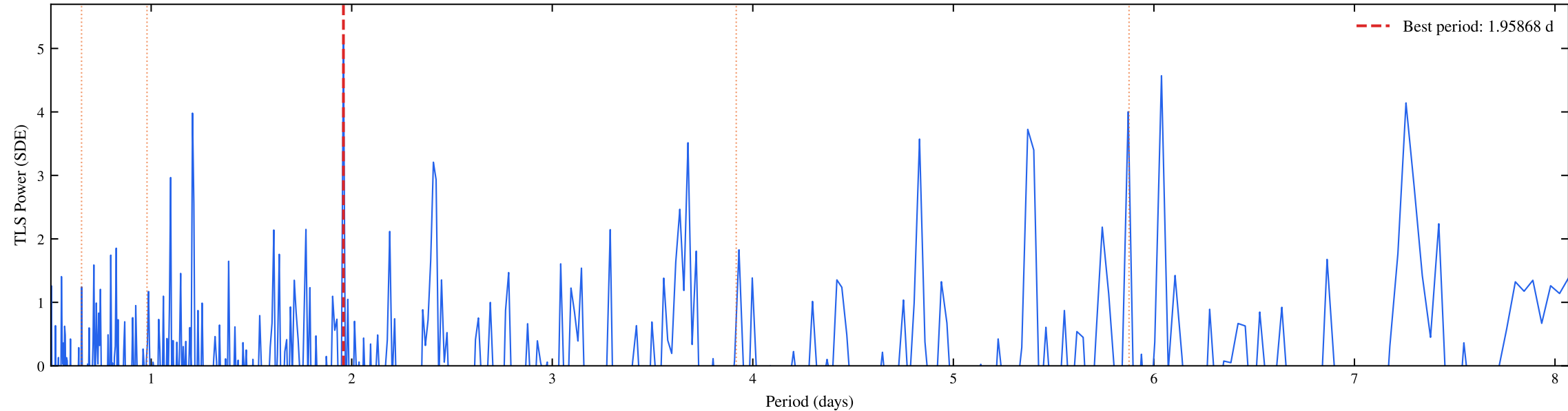
TIC 469782185 | Sectors: 67 | TLS Coarse Periodogram (SDE = 5.18)
