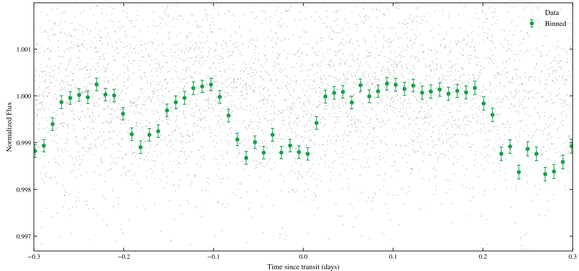
TIC 469782185 | Sectors: 67 | Phase-Folded Transit (P = 1.95902 d)
