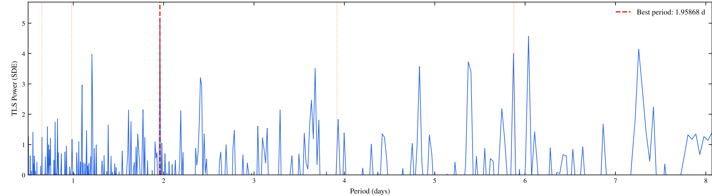
TIC 469782185 | Sectors: 67 | TLS Periodogram (Planet 2 Search) (SDE = 5.18)
