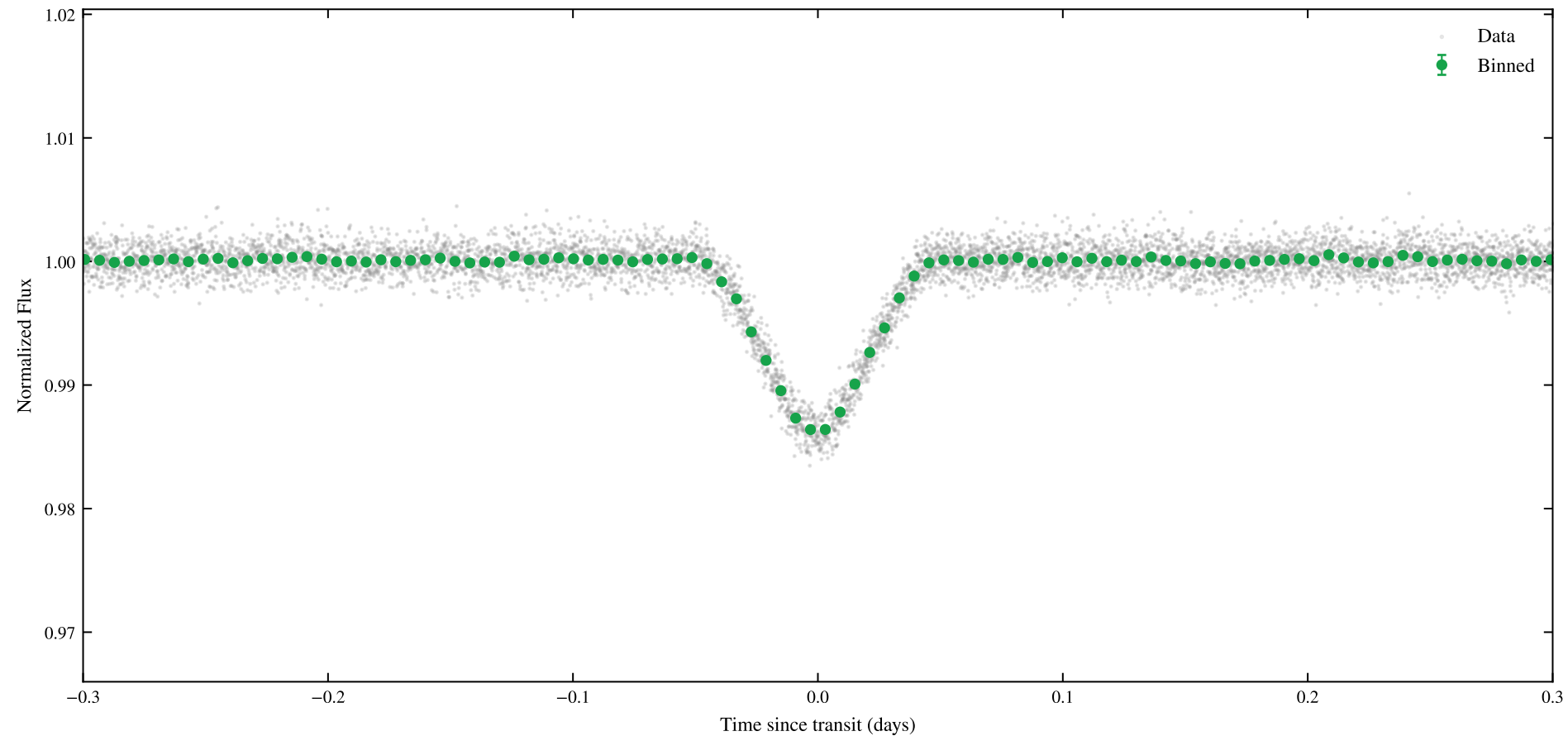
TIC 469782185 | Sectors: 67 | Phase-Folded Transit (P = 1.20936 d)
