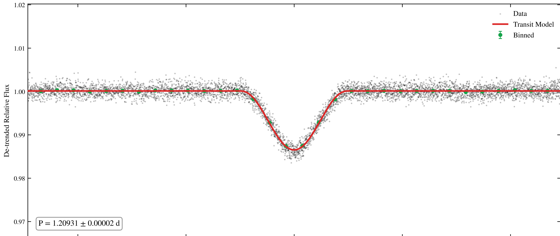
TIC 469782185 | Sectors: 67 | Phased MCMC Fit - Planet 1
