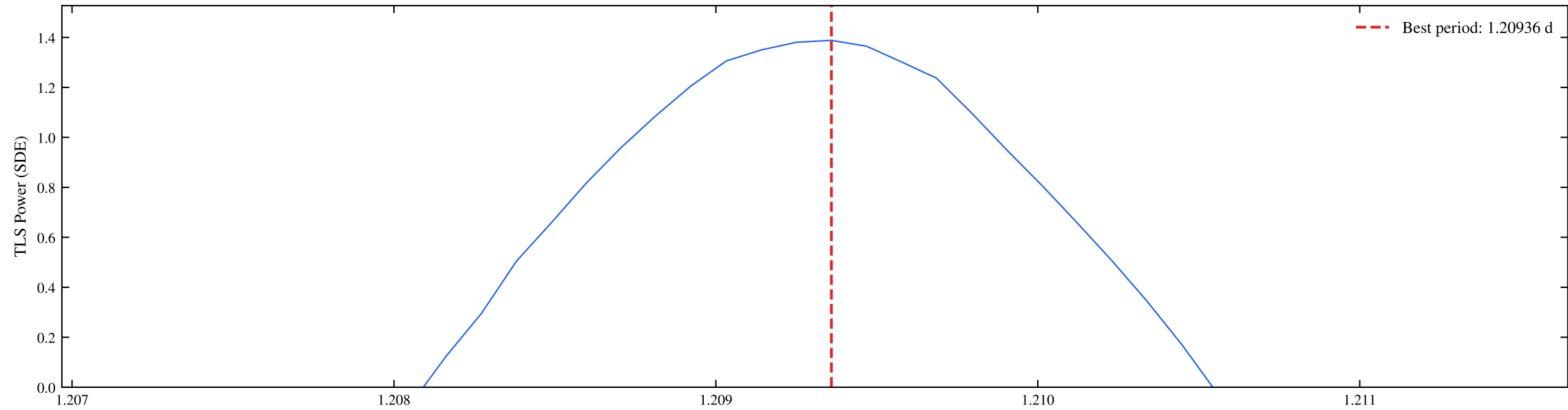
TIC 469782185 | Sectors: 67 | TLS Periodogram (Planet 2 Search) (SDE = 5.18)
