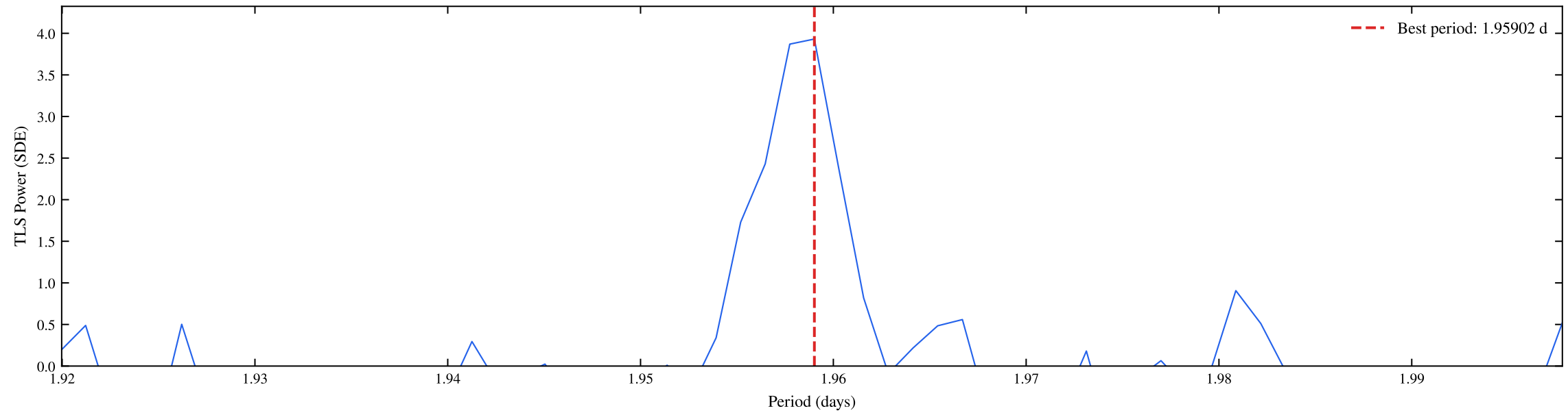
TIC 469782185 | Sectors: 67 | TLS Fine Periodogram (SDE = 3.93)
