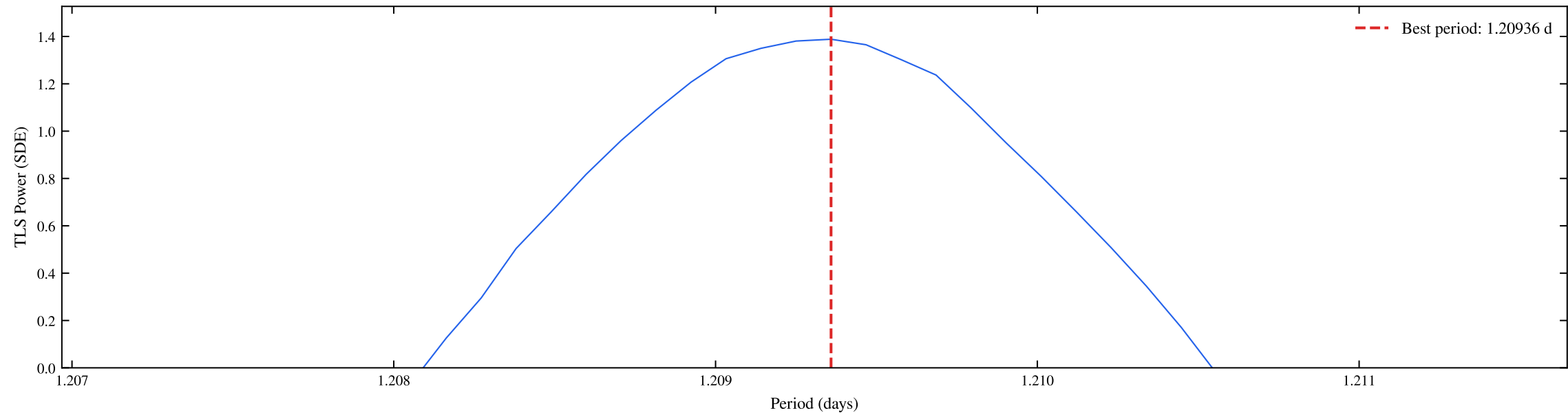
TIC 469782185 | Sectors: 67 | TLS Fine Periodogram (SDE = 1.39)
