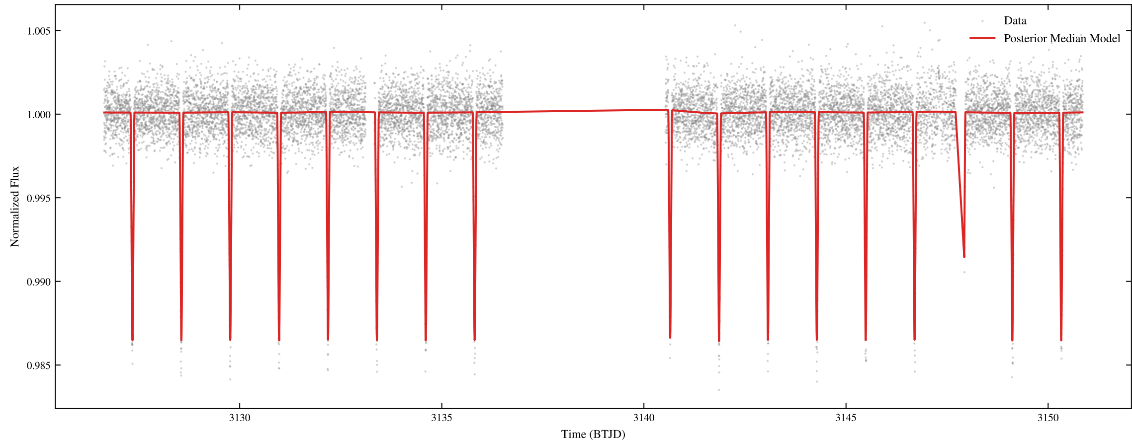
TIC 469782185 | Sectors: 67 | MCMC Posterior Predictive Check
