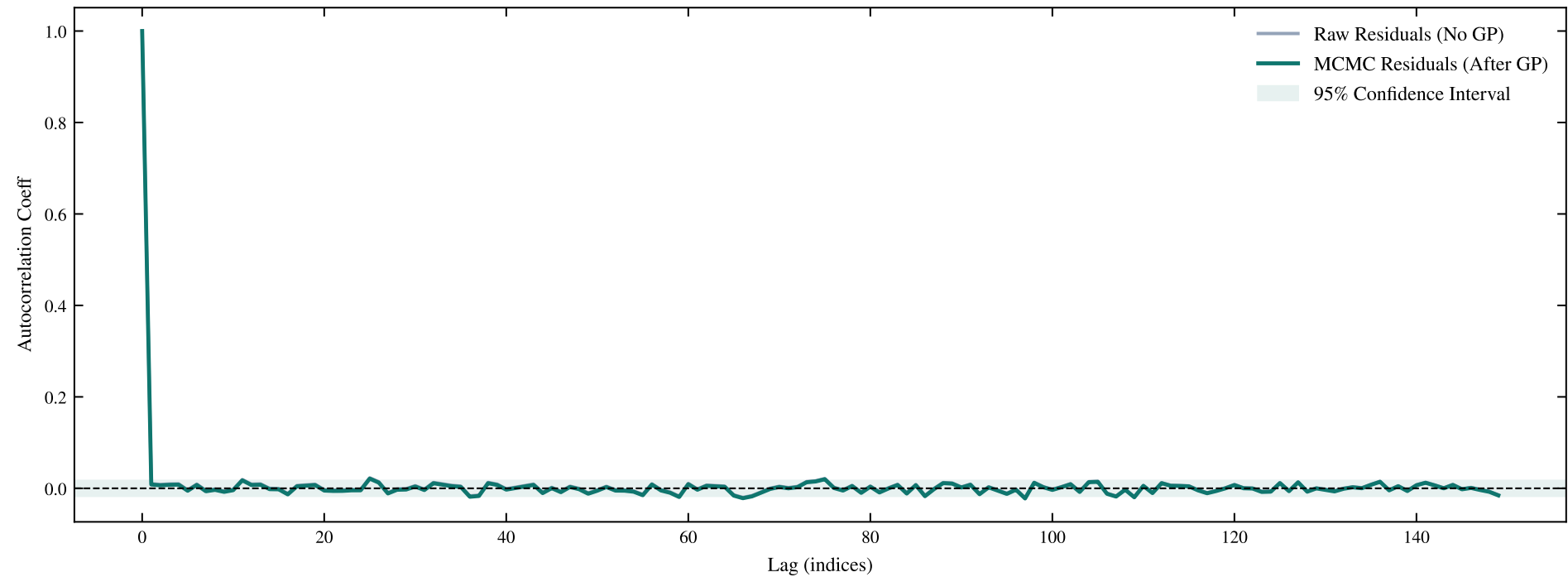
TIC 469782185 | Sectors: 67 | GP Residuals Autocorrelation Function (ACF)
